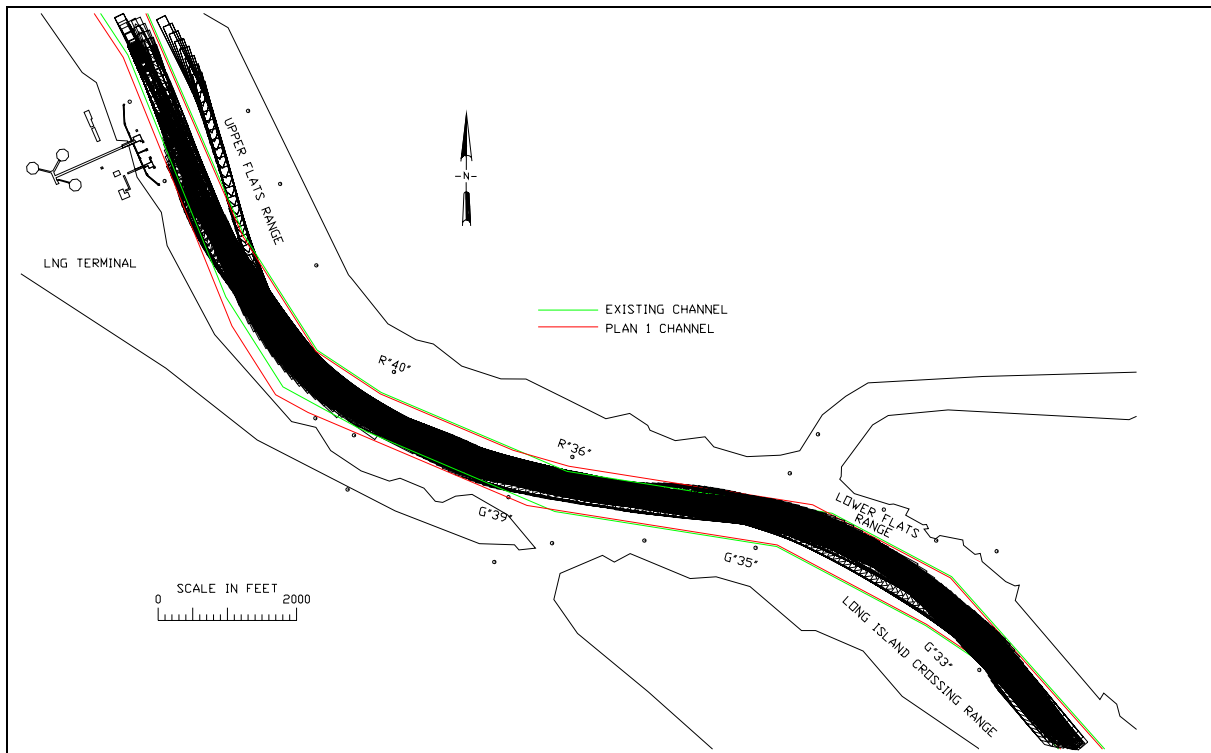
Figure 20. Composite plot of all S-class runs through Flats Range area wideners
