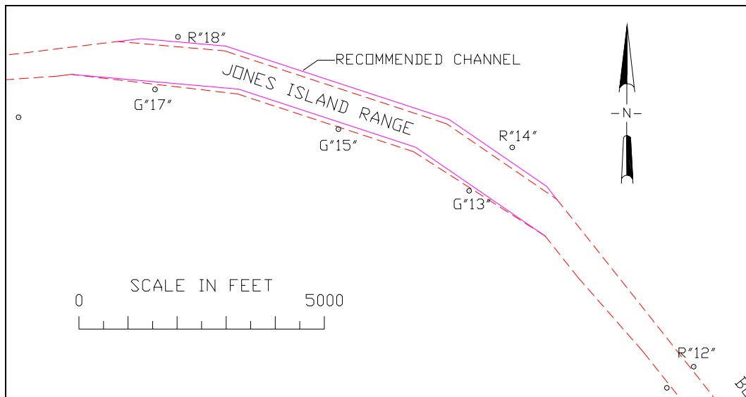
Figure 26. Recommended widener for Jones Island Range
