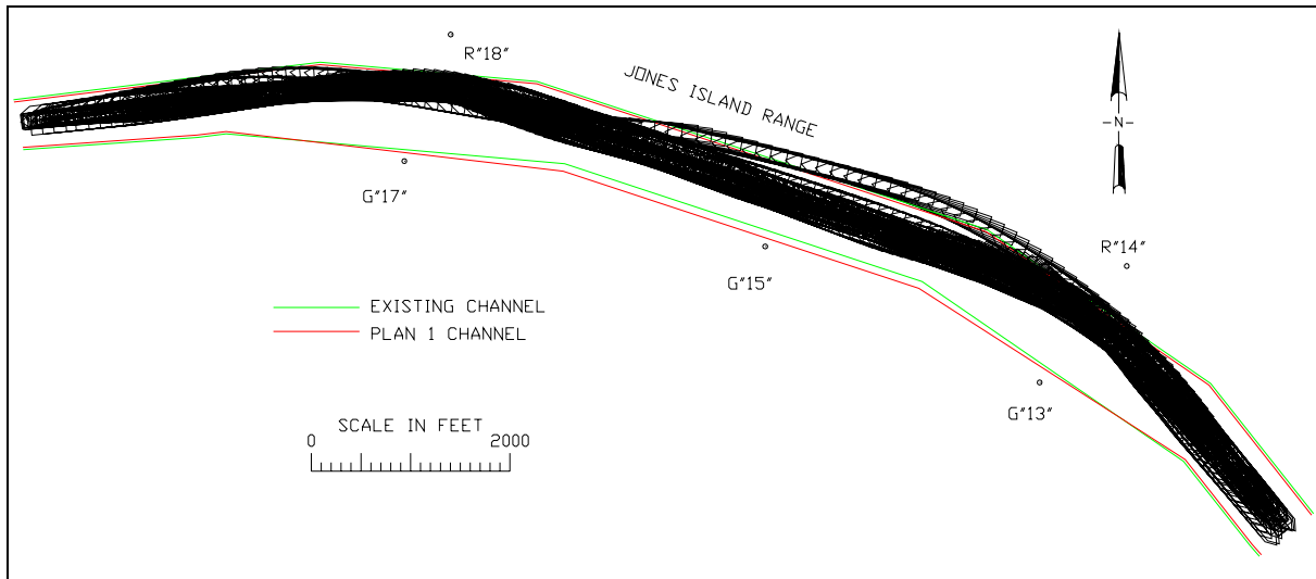
Figure 17. Jones Island Range – all S-class runs
