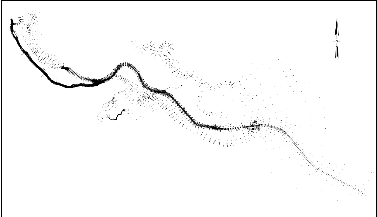
Figure 12. Flood-tidal currents
