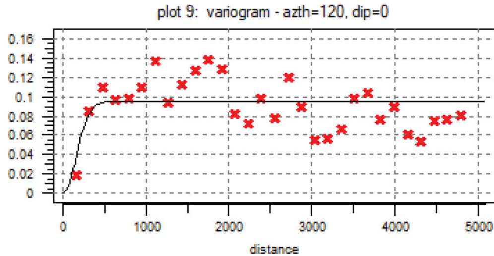
(A) Maximum Correlation Length 912 Feet at Azimuth 30 degrees (B) Minimum Correlation Length 384 Feet at Azimuth 120 degrees. Variance = 0.095, Nugget Variance = 0. Fit with Gaussian Variogram Model.
