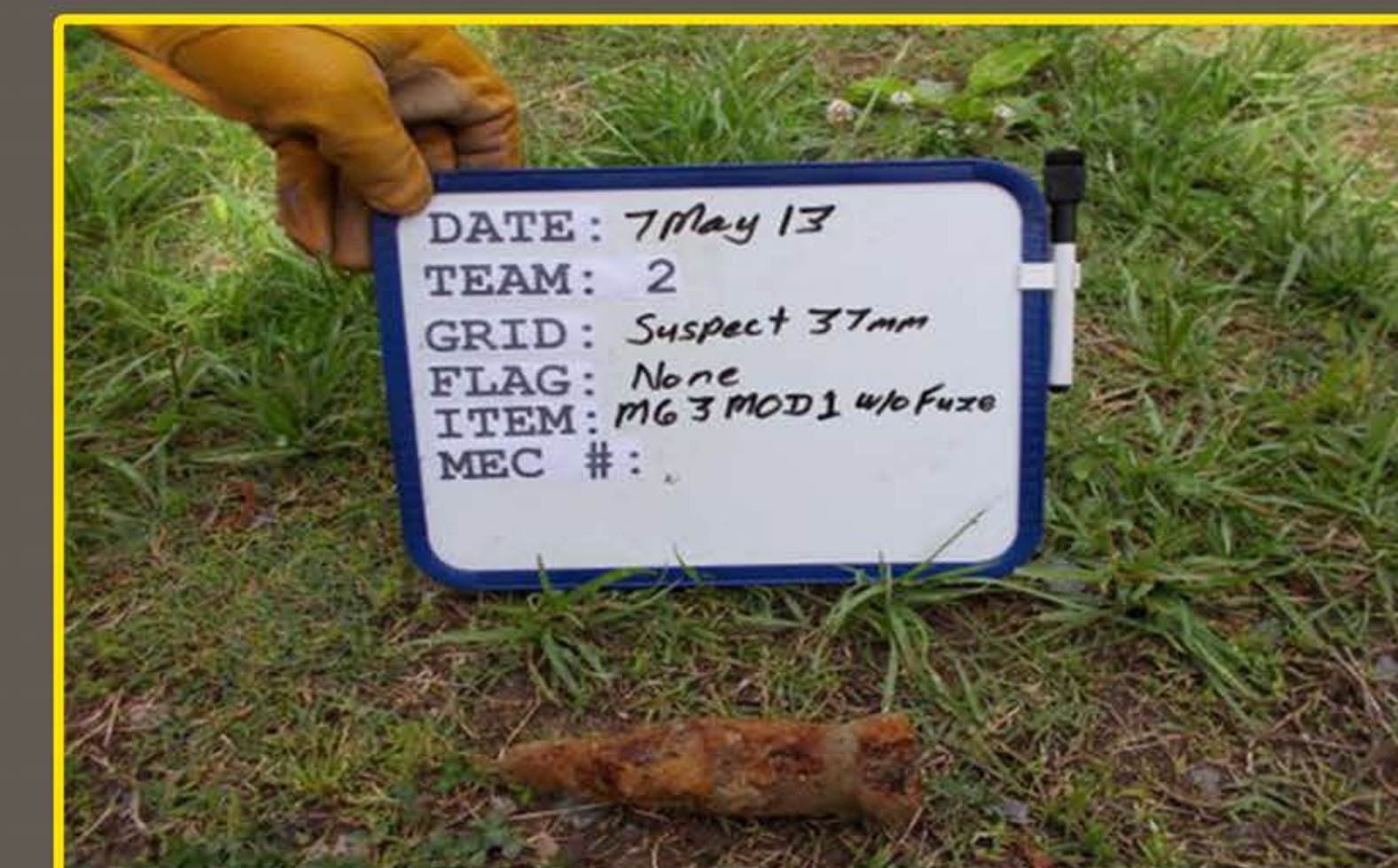
37mm Tracer Projectile
